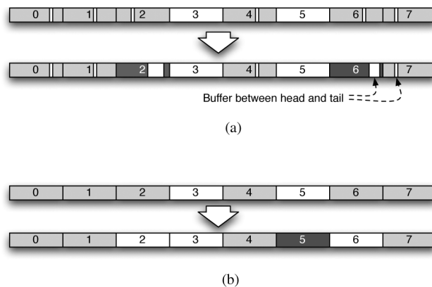
Fig. 2. Two basic layout options for SWDs [1]. (a) Bands filled with circular logs. Bands 2 and 6 are cleaned, moving their free space buffers to the right within each band, and potentially increasing the size of the buffers by not copying “dead” blocks from tail to head. (b) Bands treated as segments. Bands 2 and 6 are cleaned into Band 5, allowing them to be freed.
