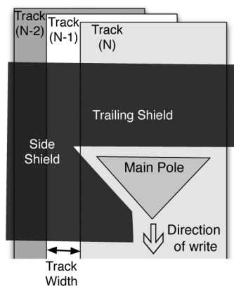
Fig. 1. Corner write head for shingled writes [1].
